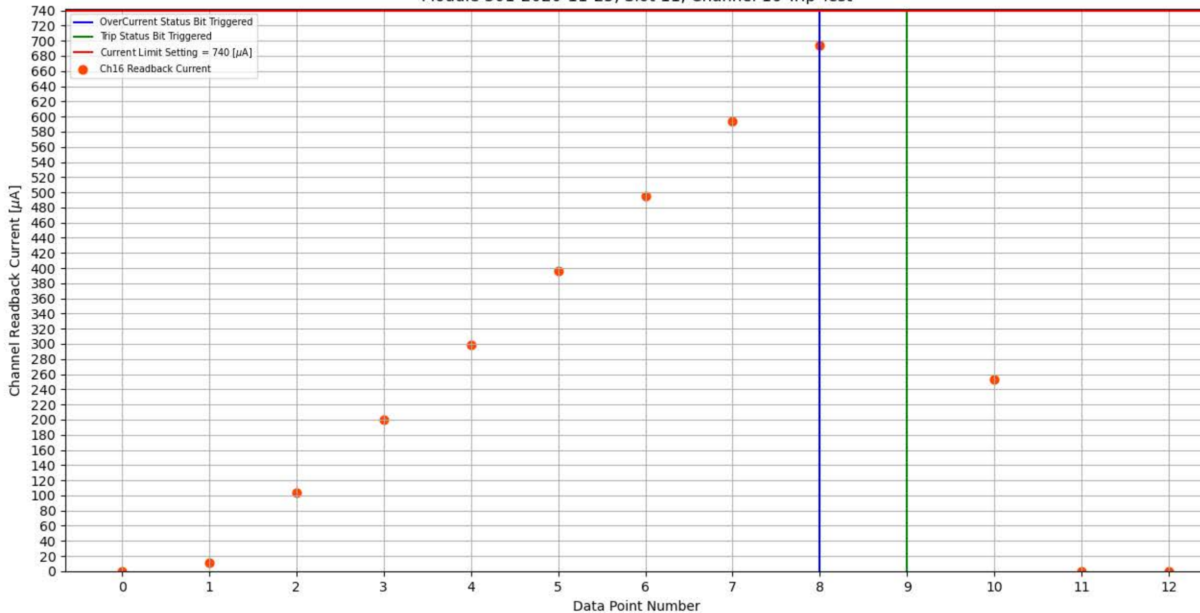
Module 301-2020-11-25, Slot 11, Channel 16 Trip Test
