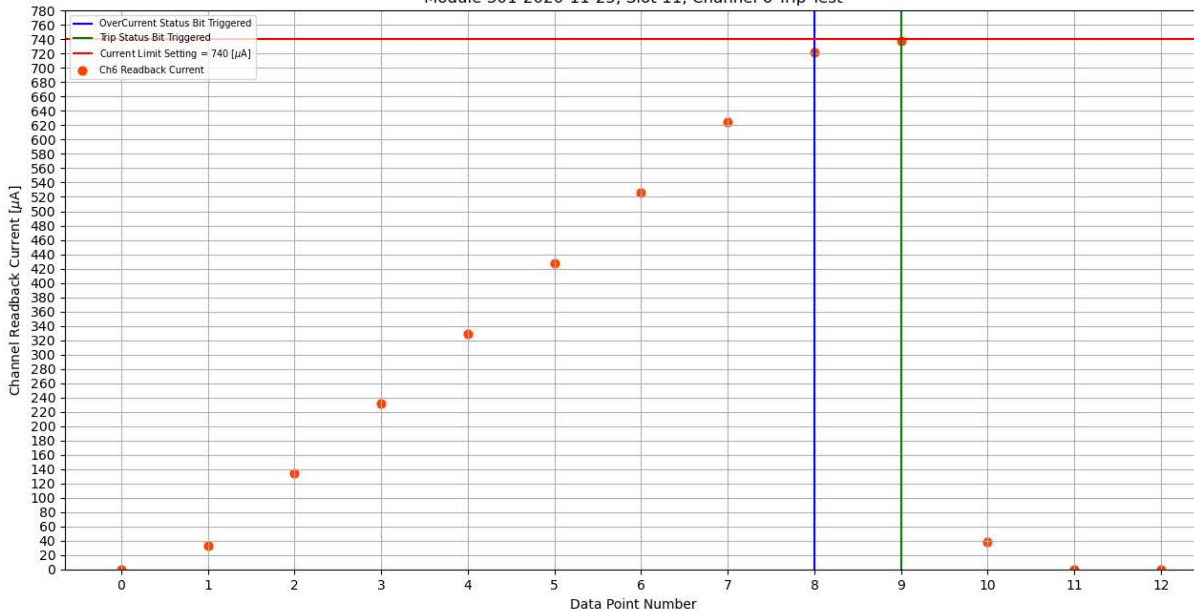
Module 301-2020-11-25, Slot 11, Channel 6 Trip Test
