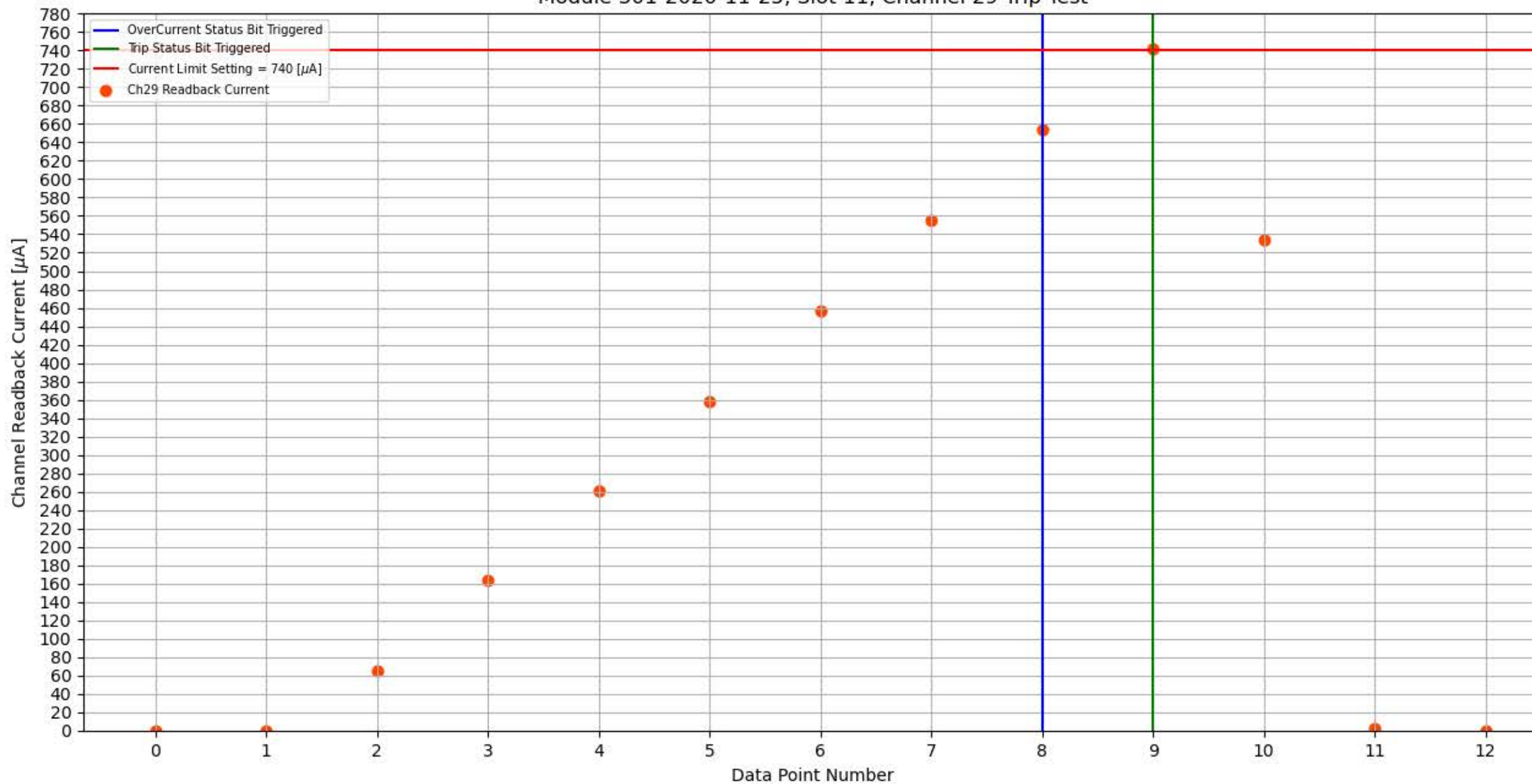
Module 301-2020-11-25, Slot 11, Channel 29 Trip Test
