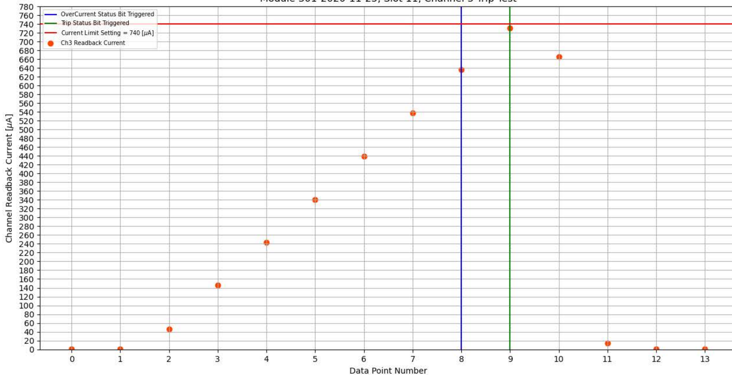
Module 301-2020-11-25, Slot 11, Channel 3 Trip Test
