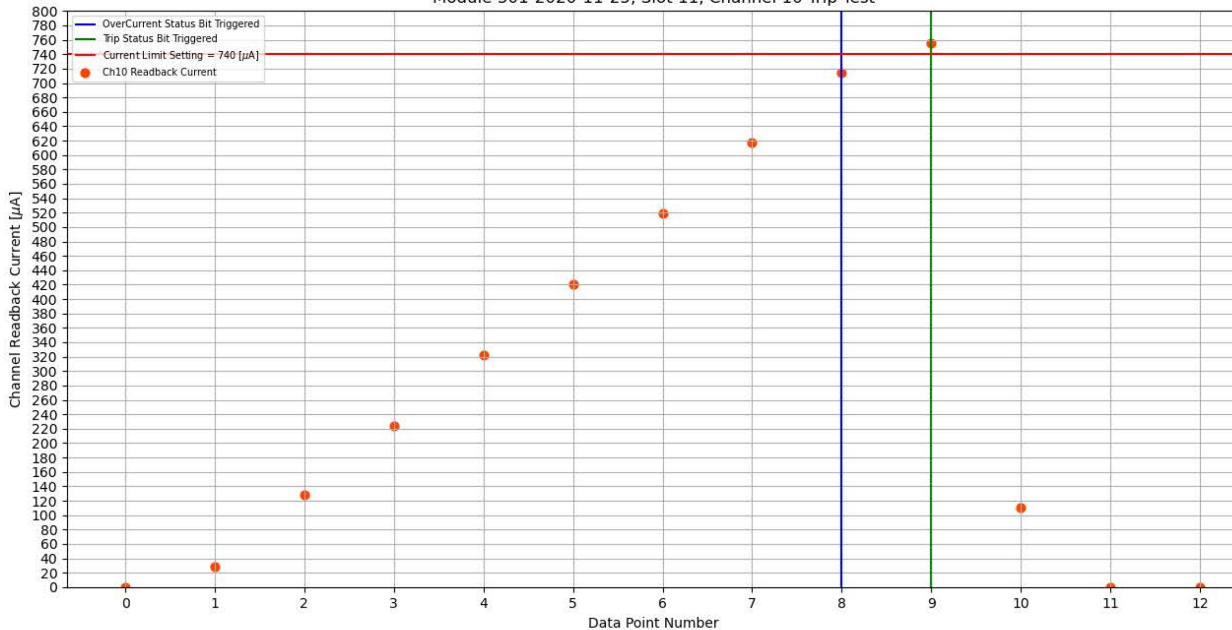
Module 301-2020-11-25, Slot 11, Channel 10 Trip Test
