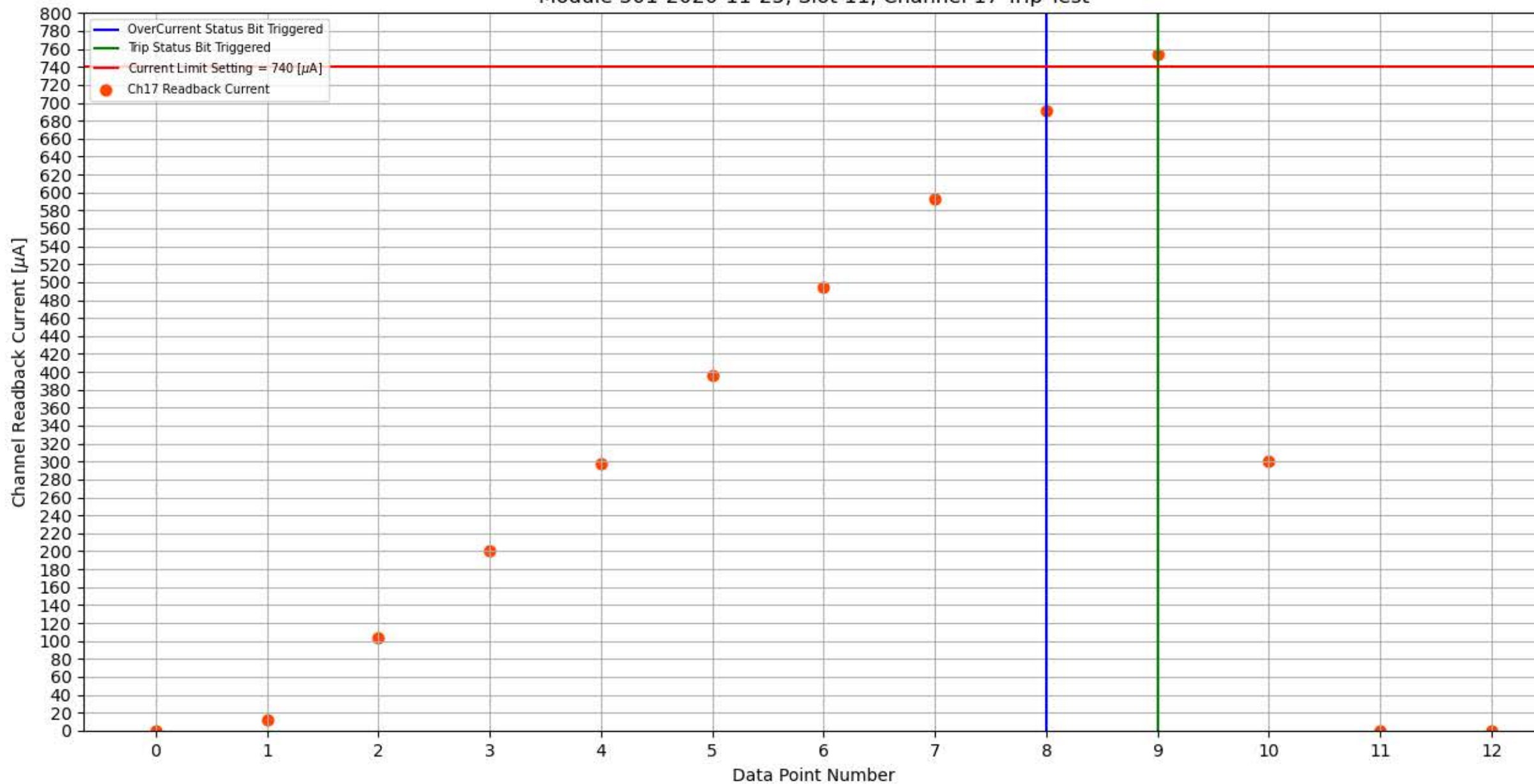
Module 301-2020-11-25, Slot 11, Channel 17 Trip Test
