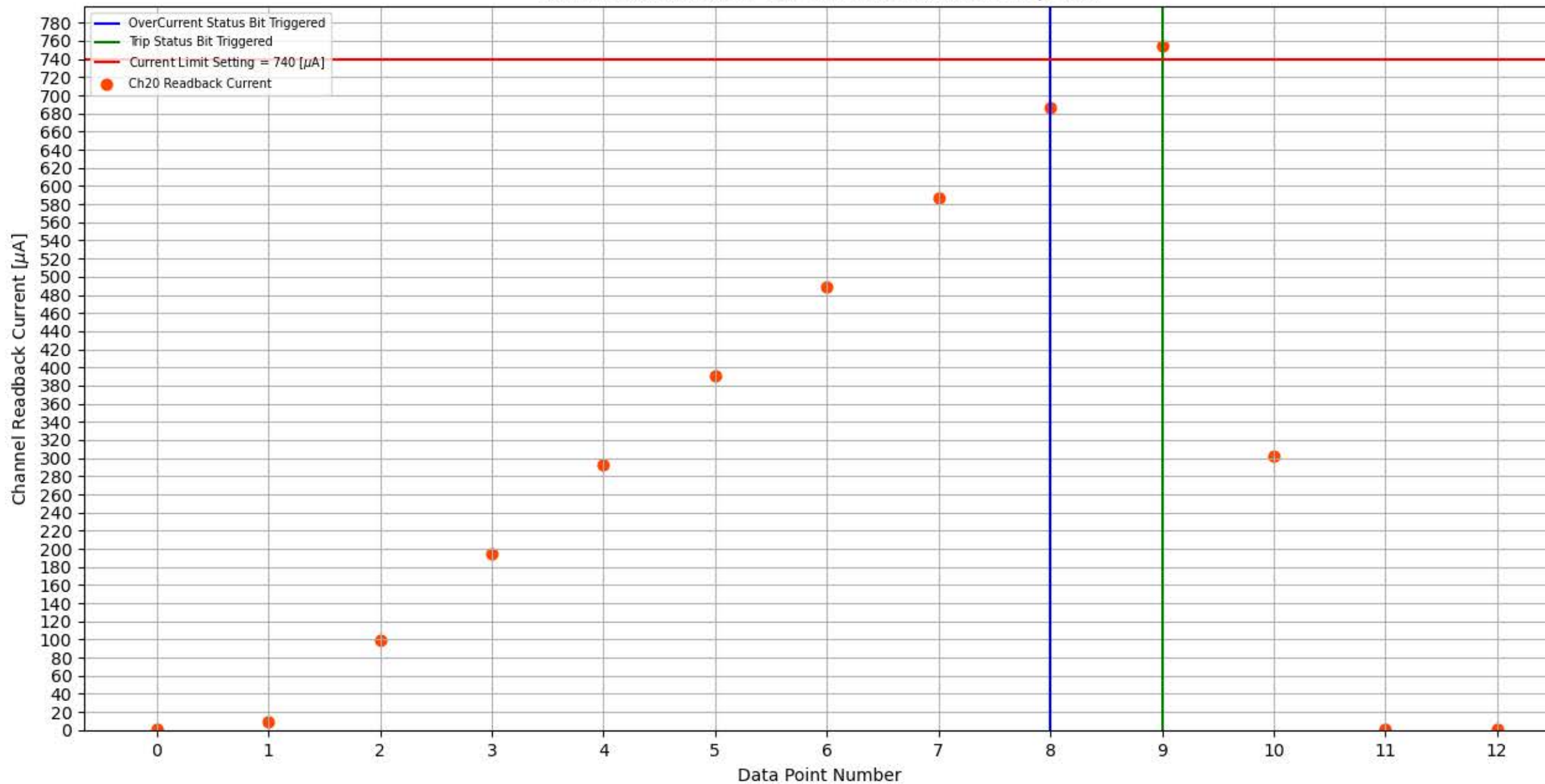
Module 301-2020-11-25, Slot 11, Channel 20 Trip Test
