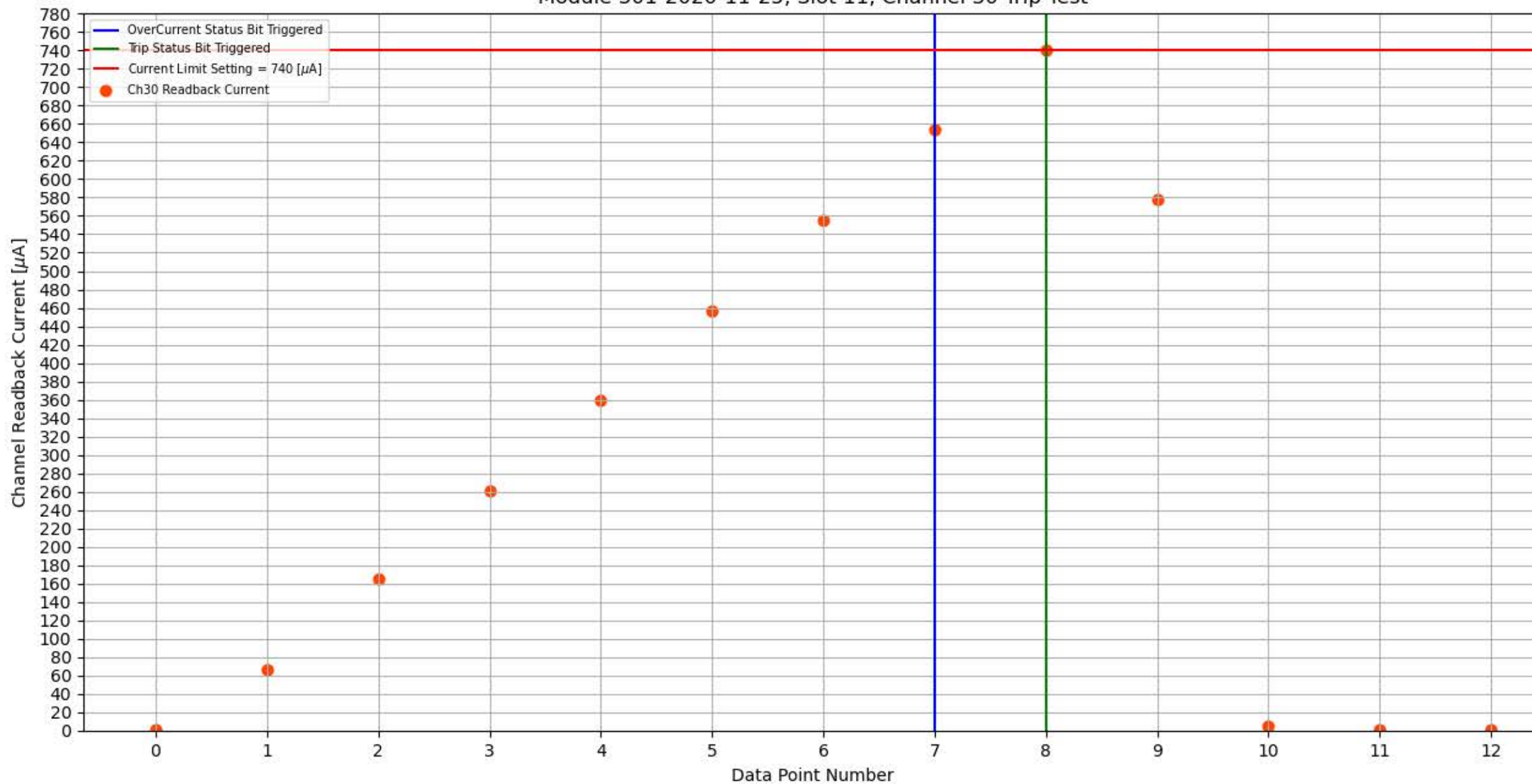
Module 301-2020-11-25, Slot 11, Channel 30 Trip Test
