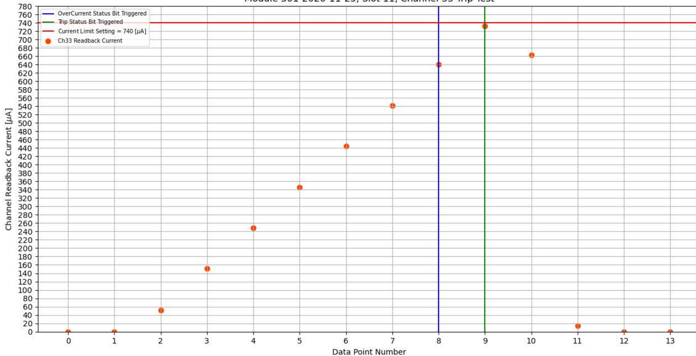
Module 301-2020-11-25, Slot 11, Channel 33 Trip Test
