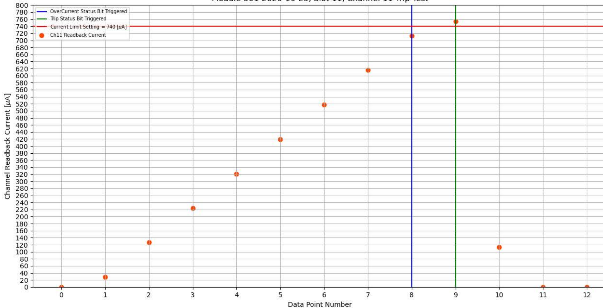
Module 301-2020-11-25, Slot 11, Channel 11 Trip Test
