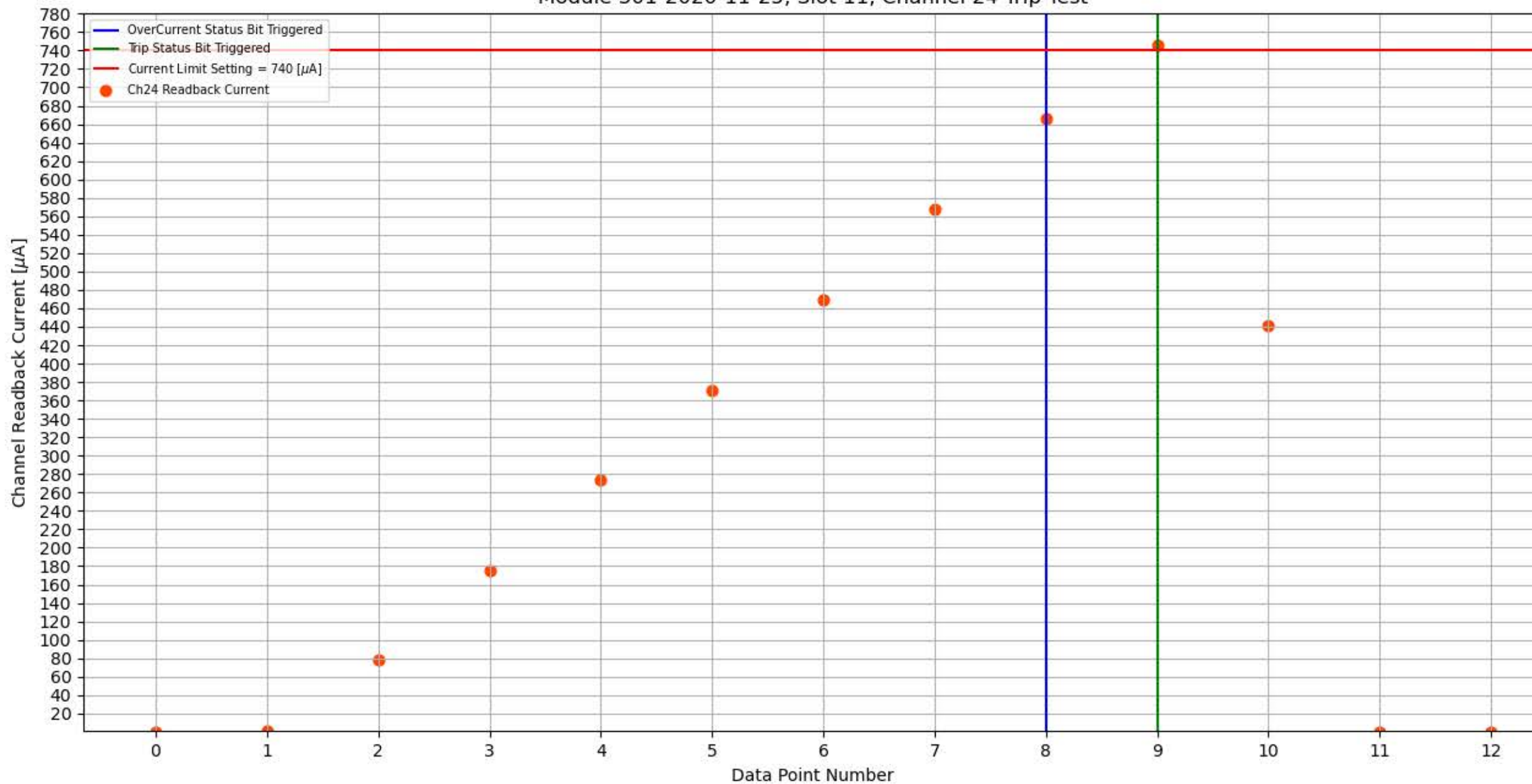
Module 301-2020-11-25, Slot 11, Channel 24 Trip Test
