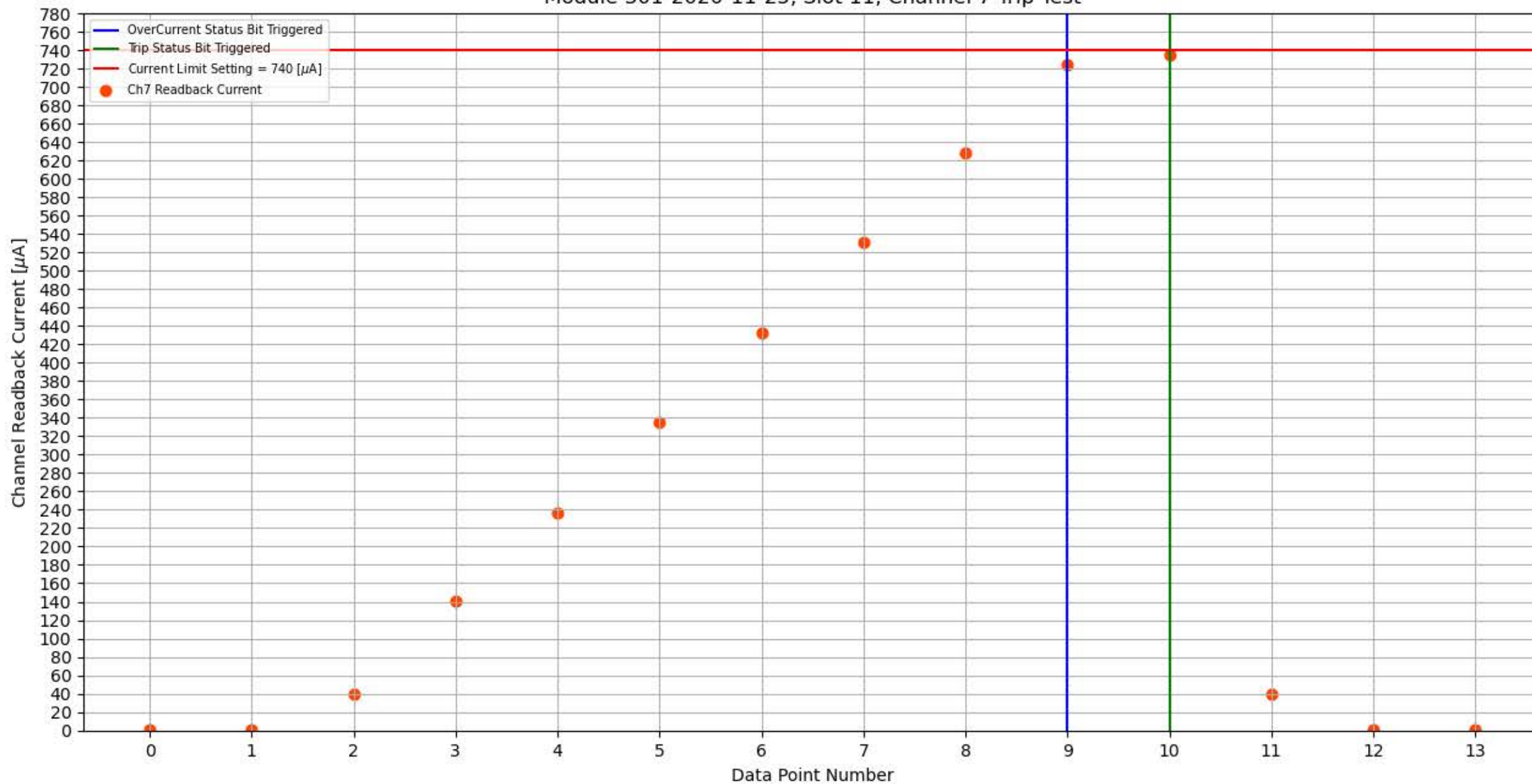
Module 301-2020-11-25, Slot 11, Channel 7 Trip Test
