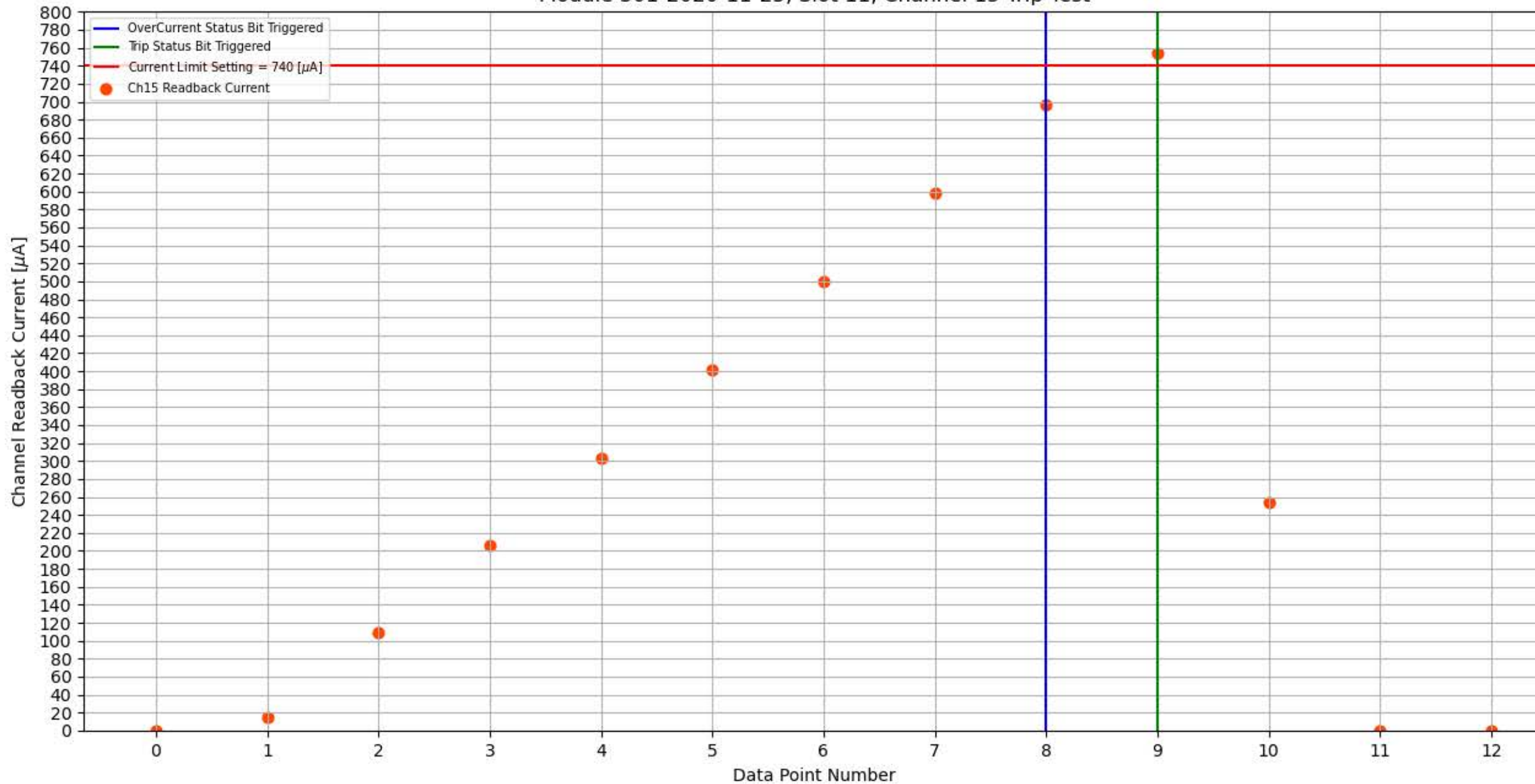
Module 301-2020-11-25, Slot 11, Channel 15 Trip Test
