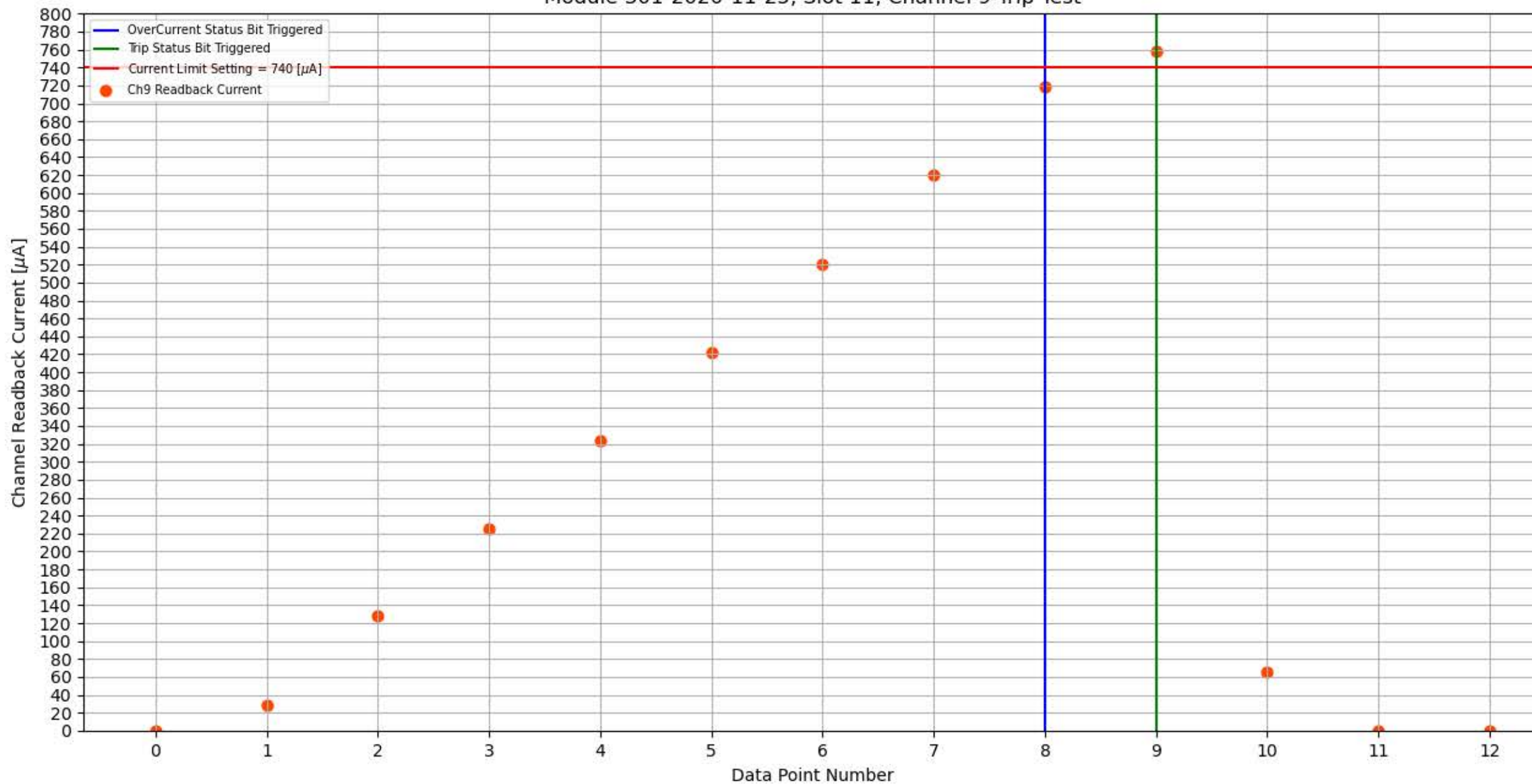
Module 301-2020-11-25, Slot 11, Channel 9 Trip Test
