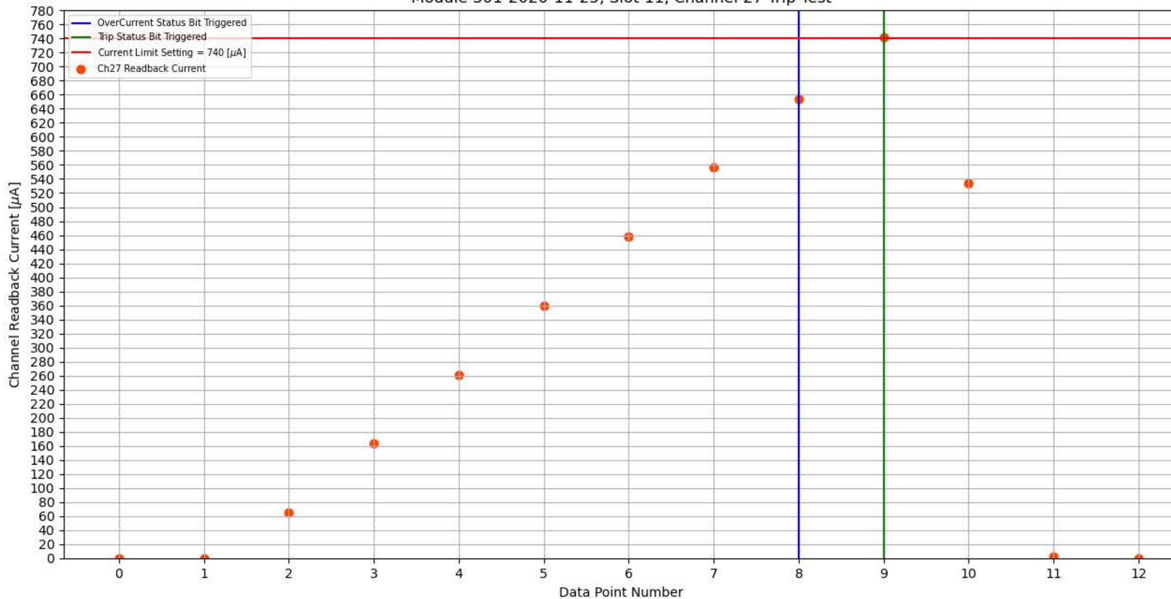
Module 301-2020-11-25, Slot 11, Channel 27 Trip Test
