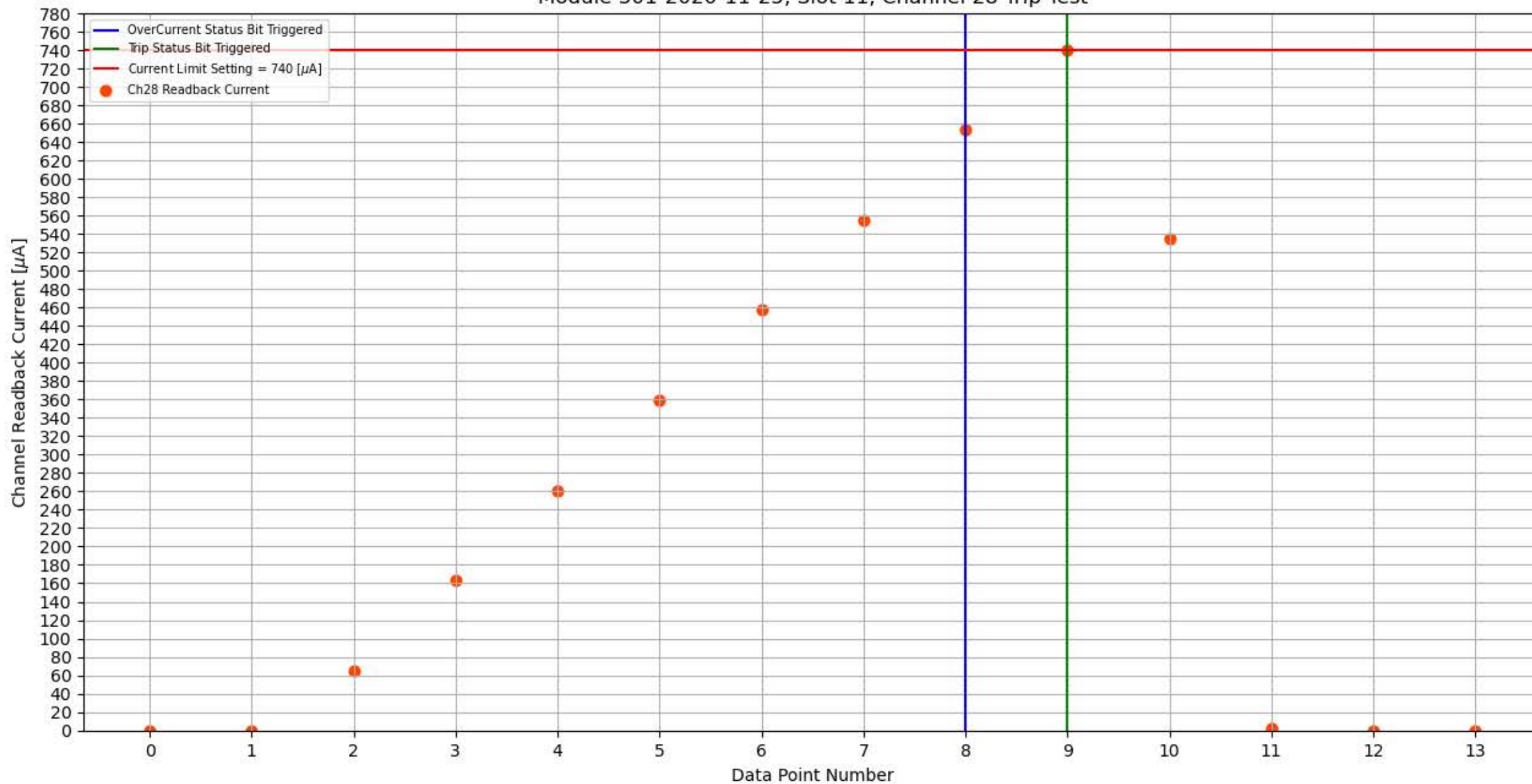
Module 301-2020-11-25, Slot 11, Channel 28 Trip Test
