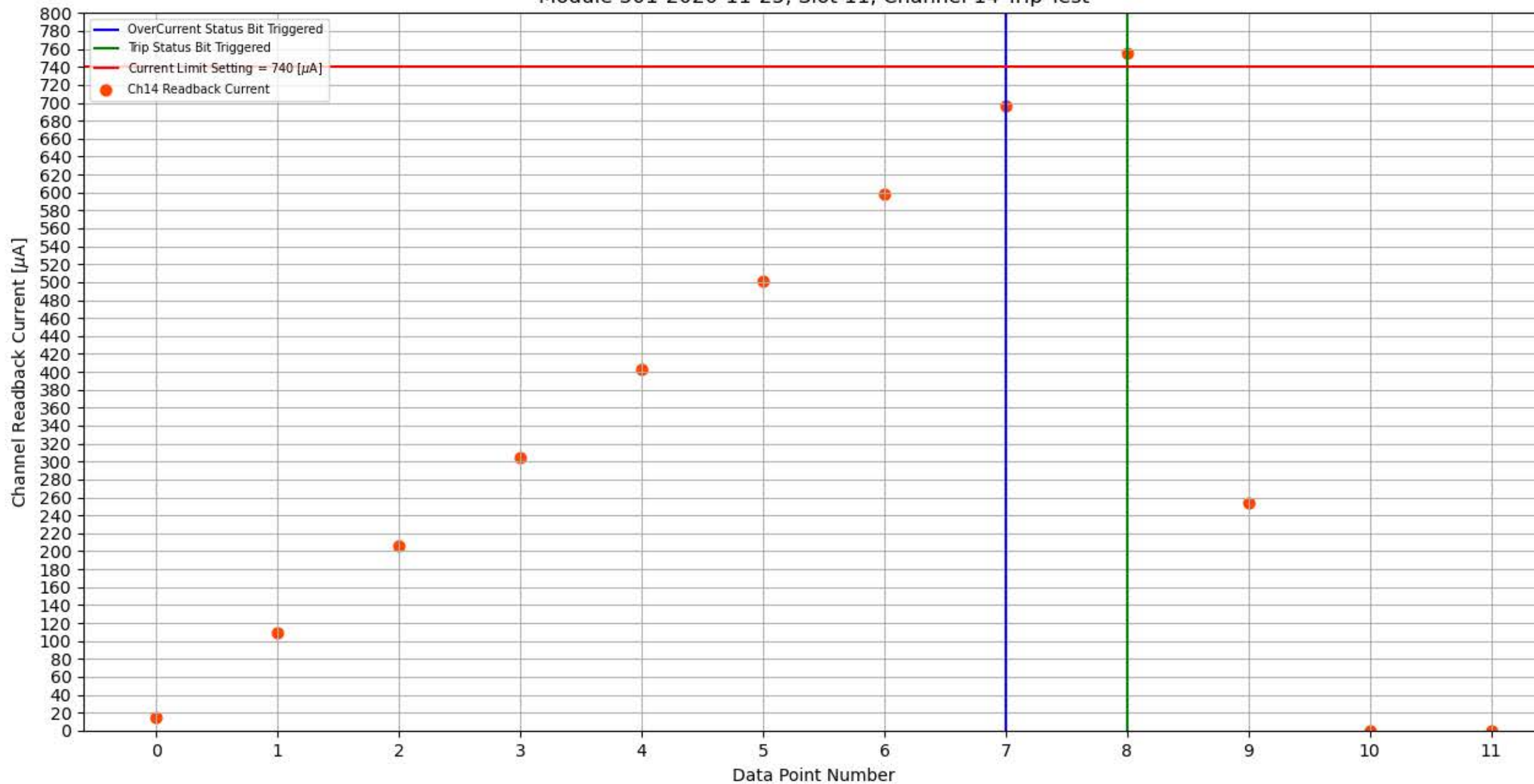
Module 301-2020-11-25, Slot 11, Channel 14 Trip Test
