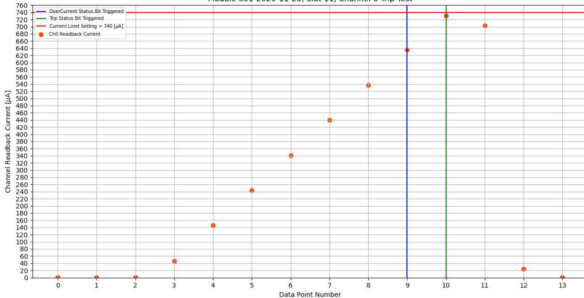
Module 301-2020-11-25, Slot 11, Channel 0 Trip Test
