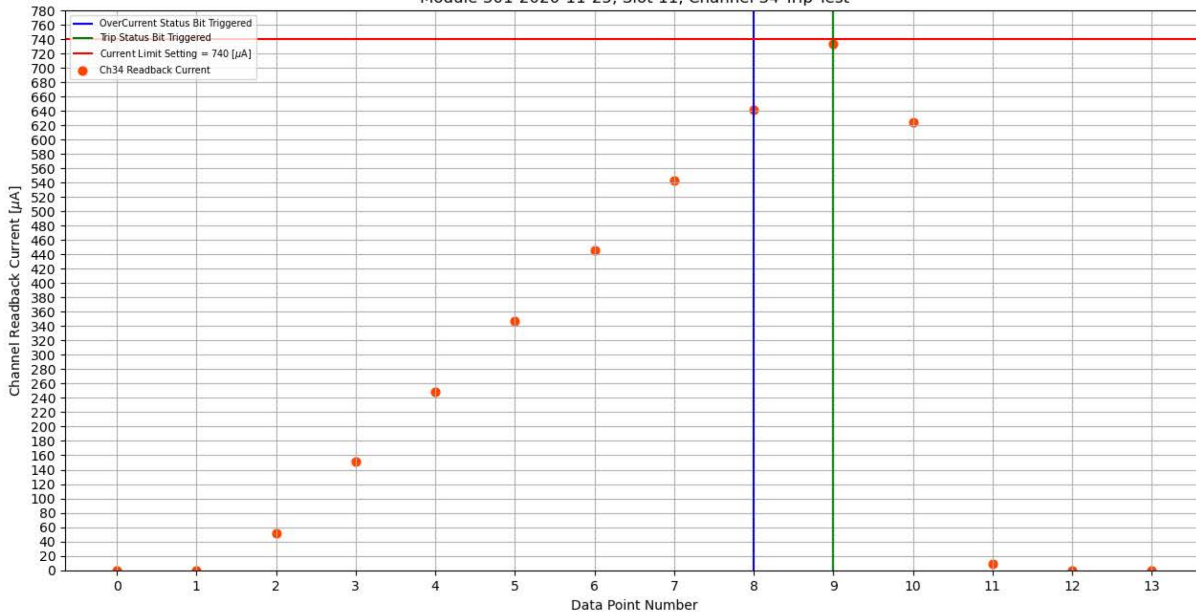
Module 301-2020-11-25, Slot 11, Channel 34 Trip Test
