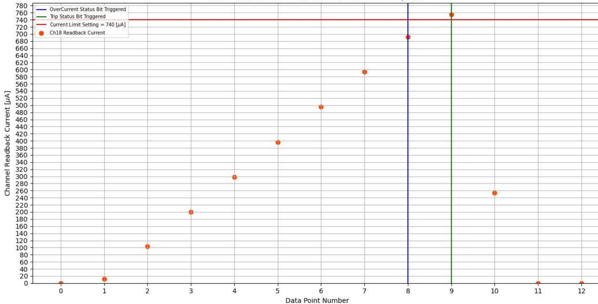
Module 301-2020-11-25, Slot 11, Channel 18 Trip Test
