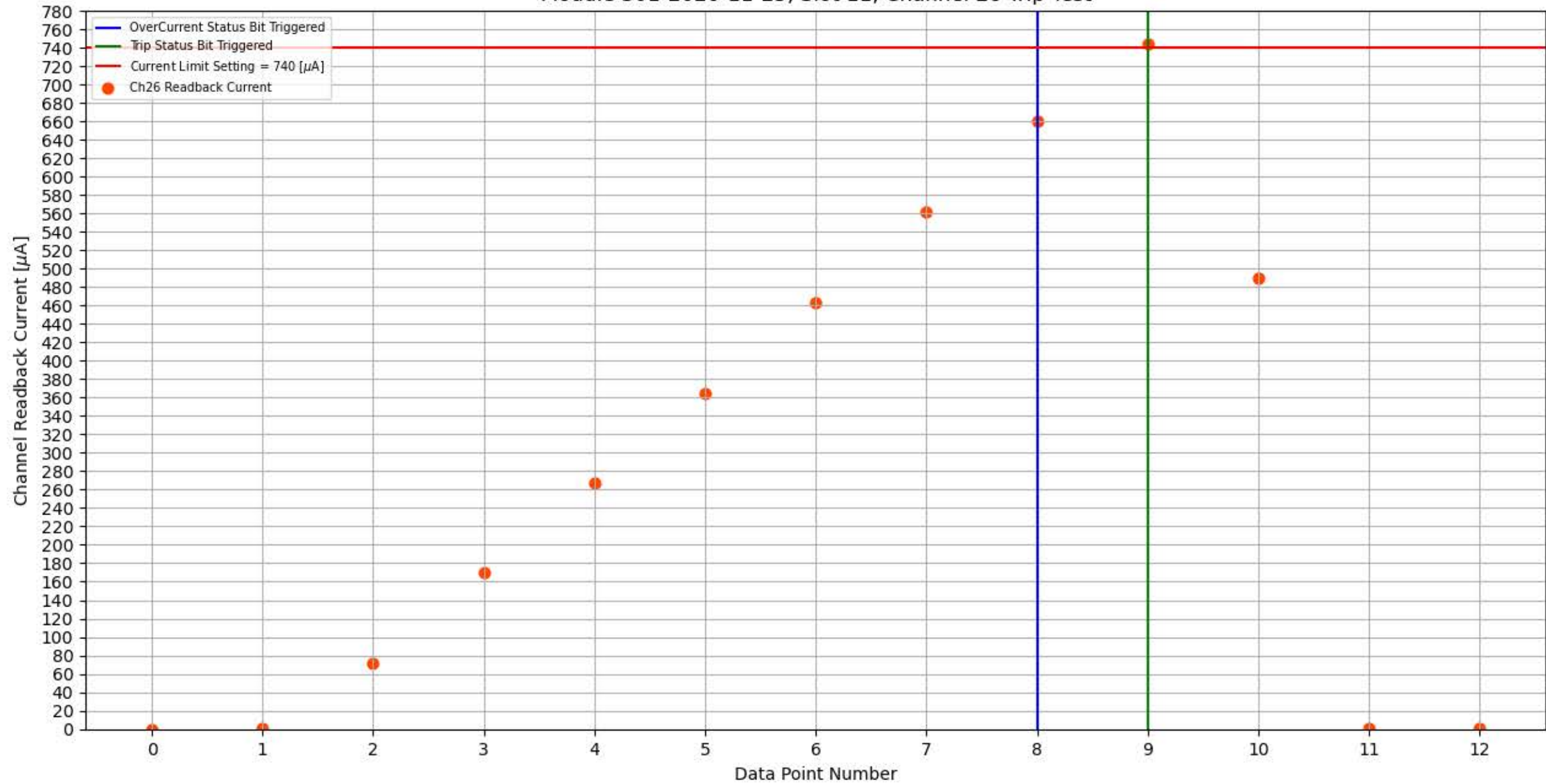
Module 301-2020-11-25, Slot 11, Channel 26 Trip Test
