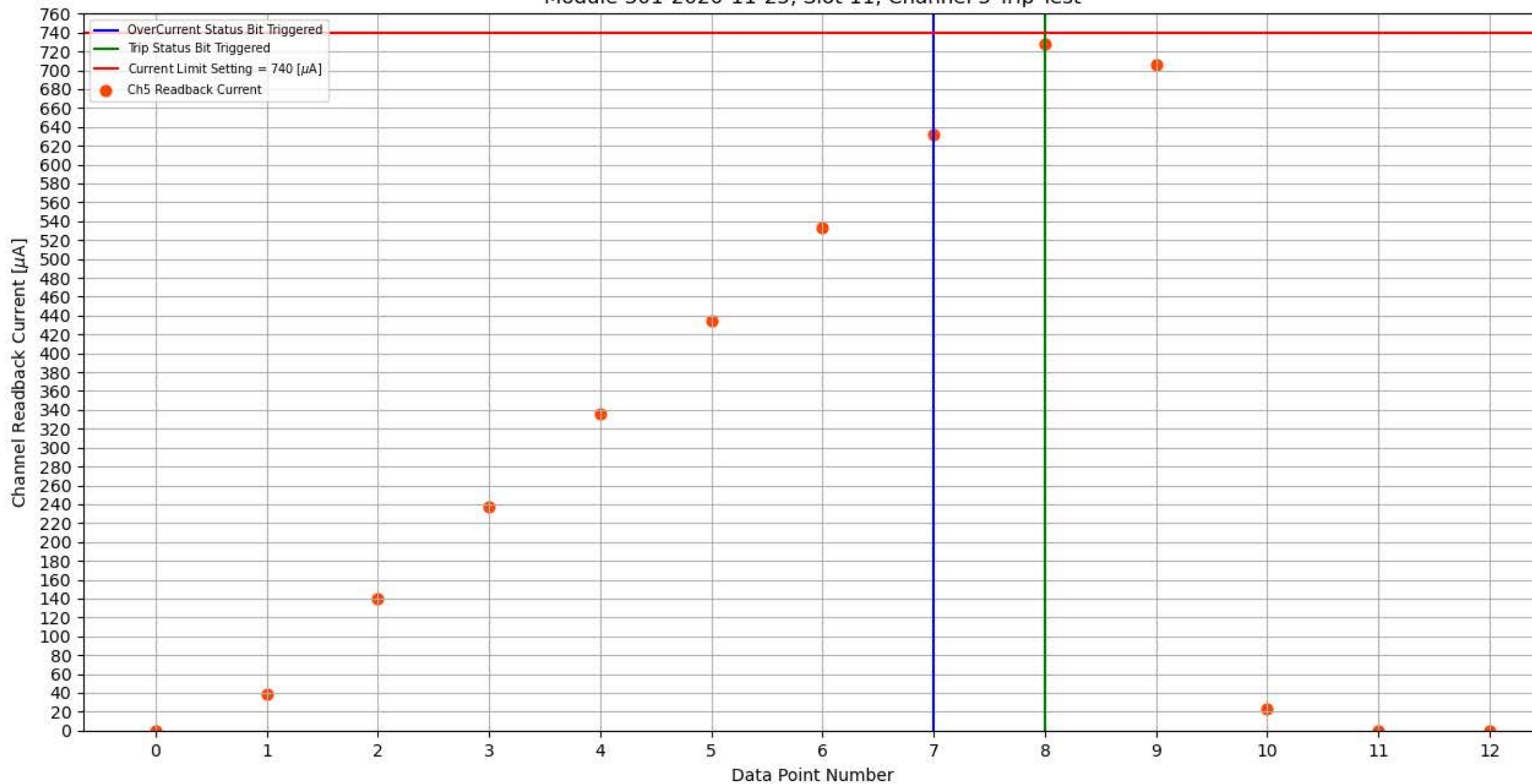
Module 301-2020-11-25, Slot 11, Channel 5 Trip Test
