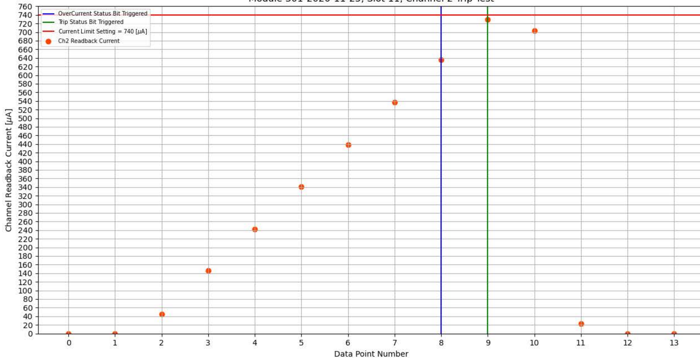
Module 301-2020-11-25, Slot 11, Channel 2 Trip Test
