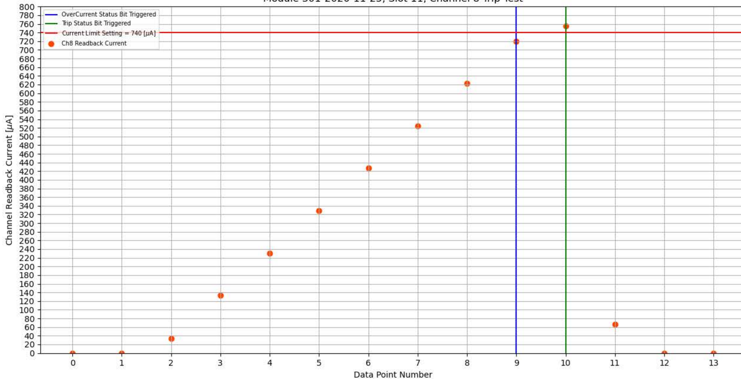
Module 301-2020-11-25, Slot 11, Channel 8 Trip Test
