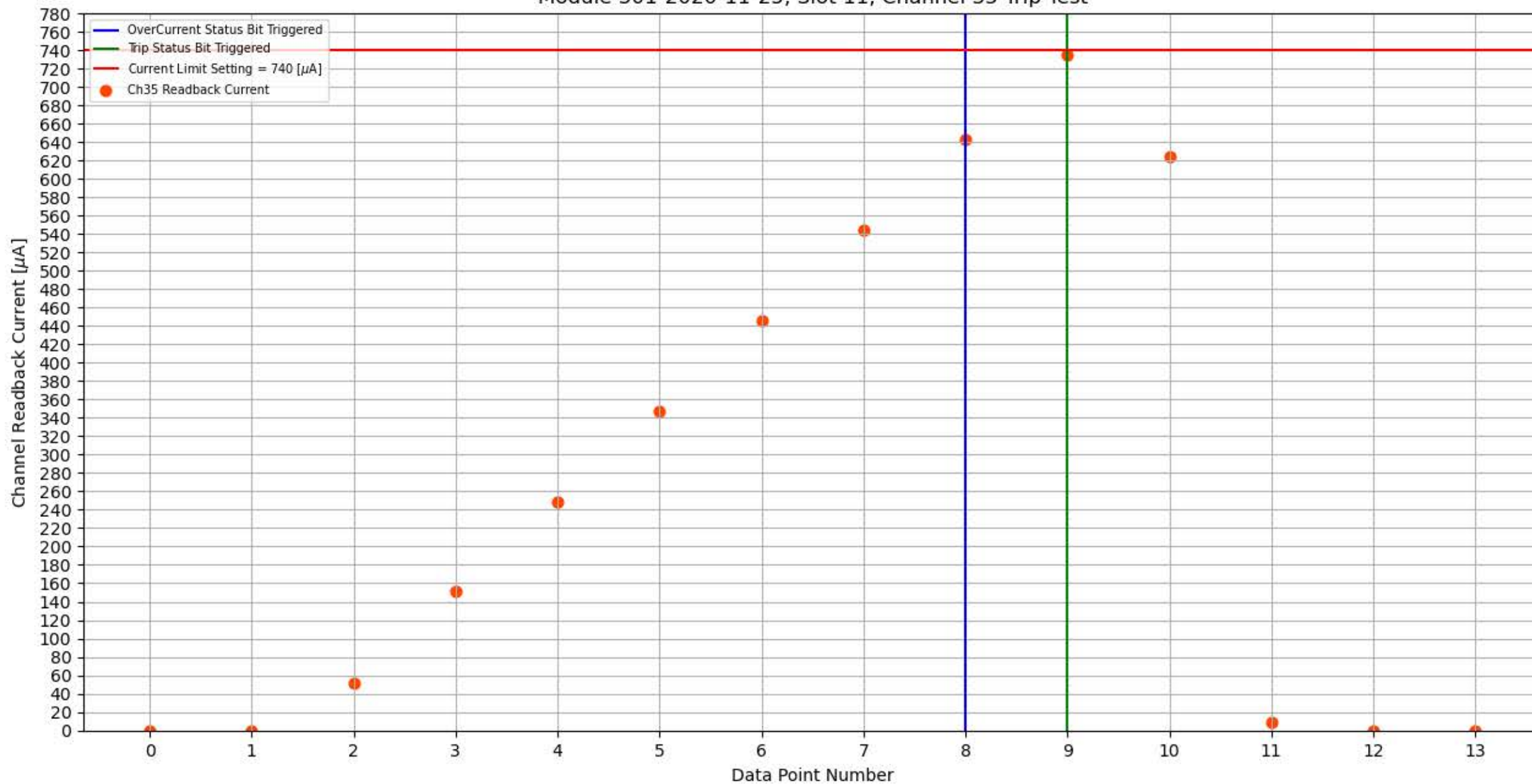
Module 301-2020-11-25, Slot 11, Channel 35 Trip Test
