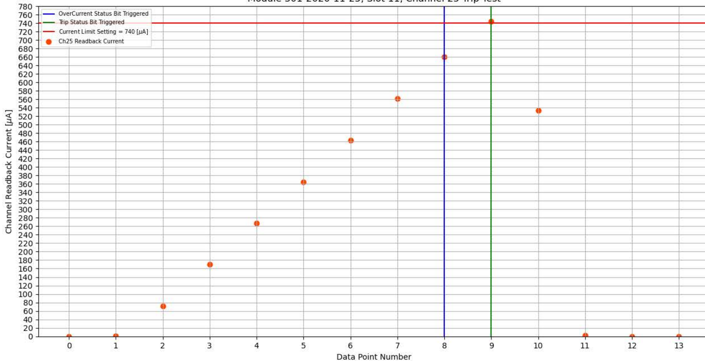
Module 301-2020-11-25, Slot 11, Channel 25 Trip Test
