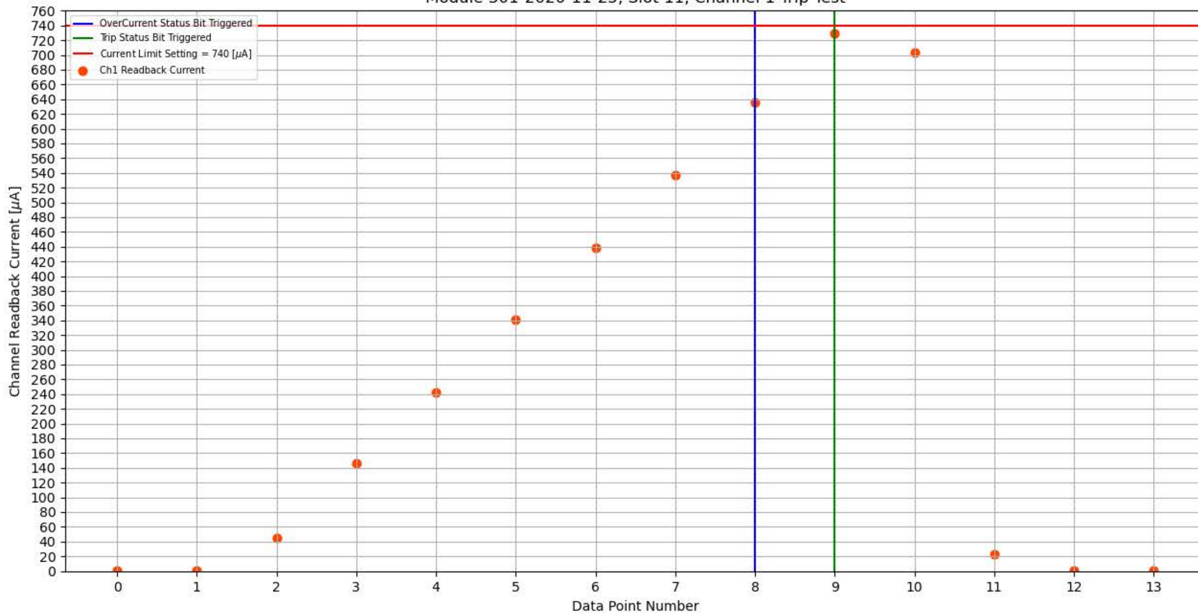
Module 301-2020-11-25, Slot 11, Channel 1 Trip Test
