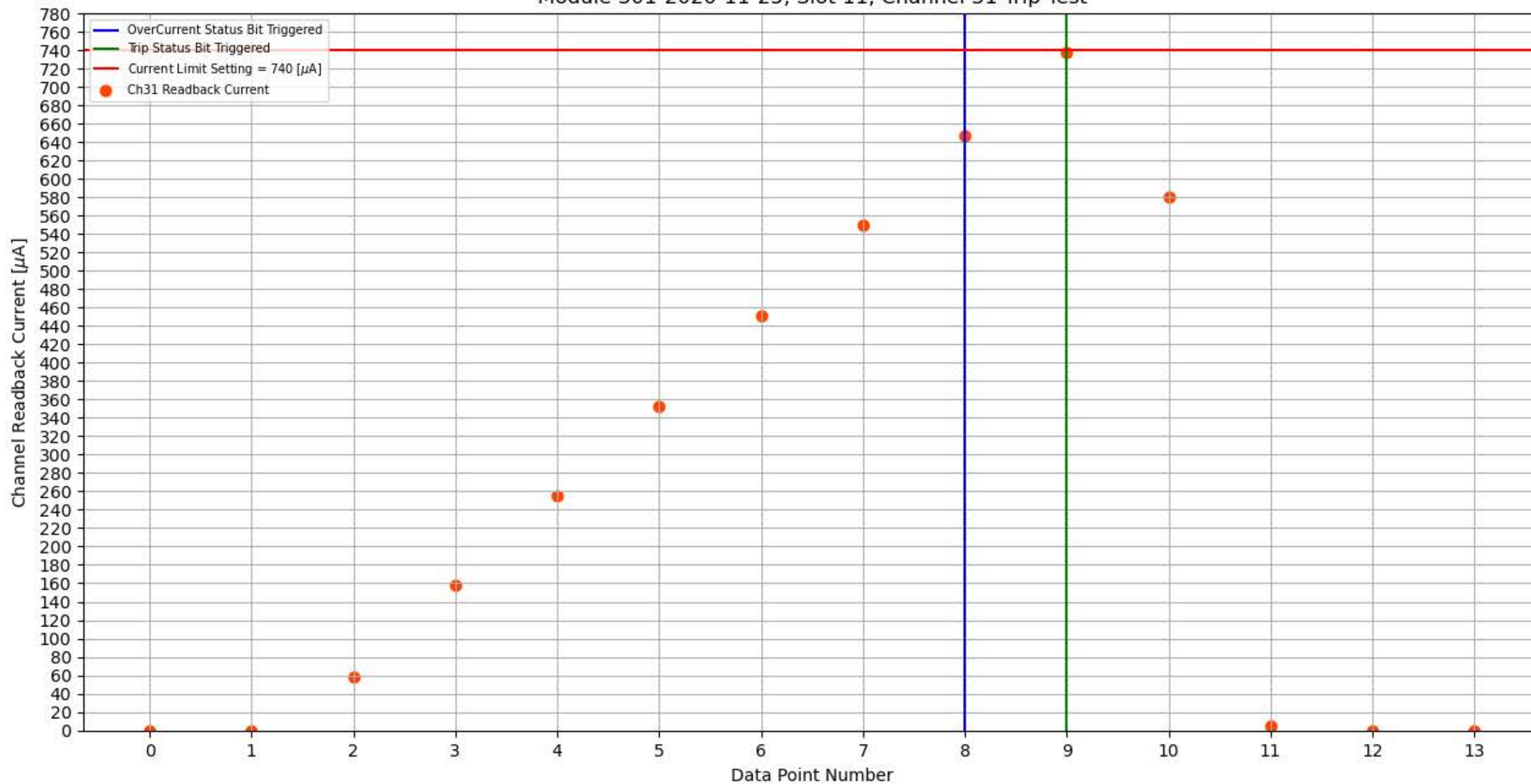
Module 301-2020-11-25, Slot 11, Channel 31 Trip Test
