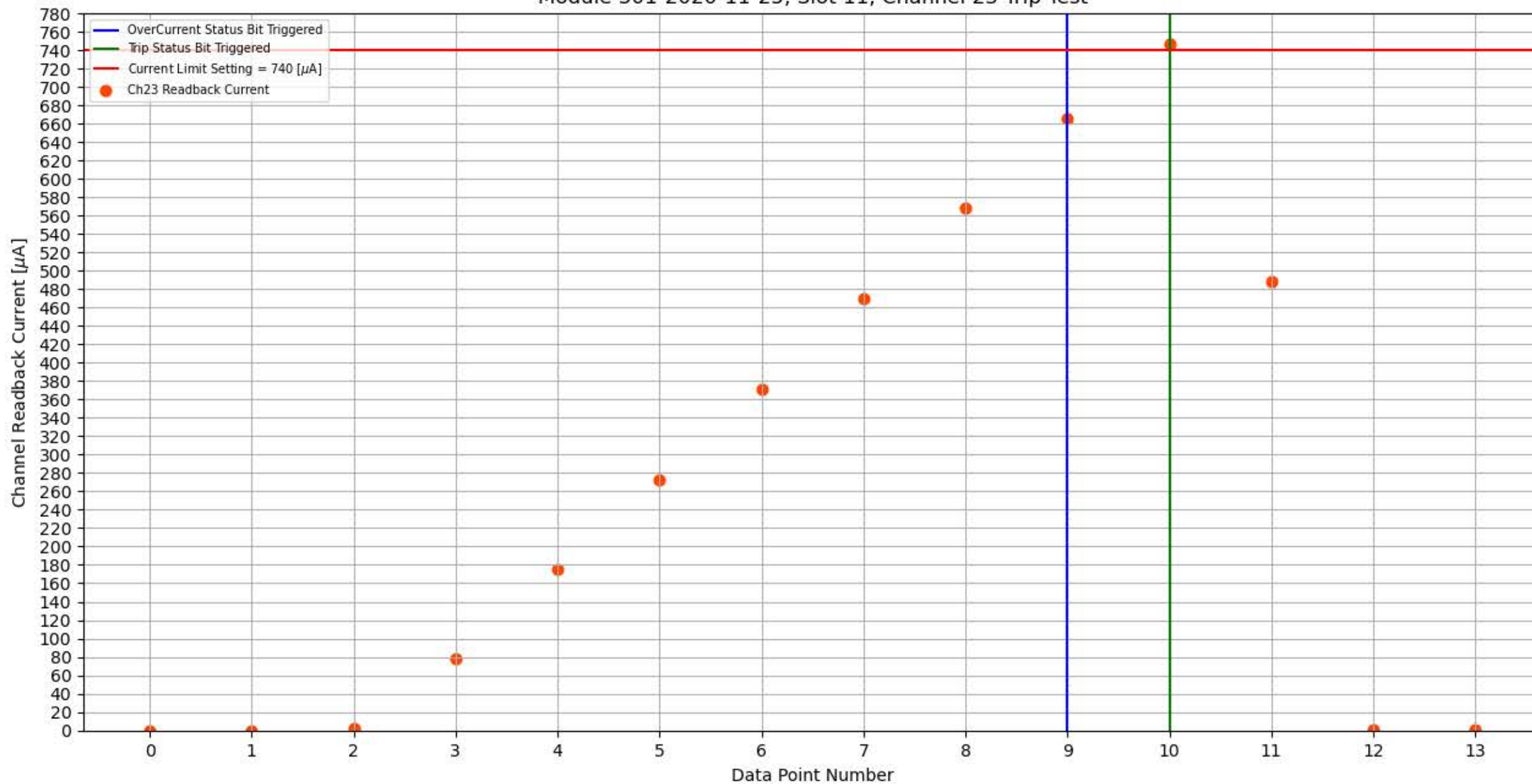
Module 301-2020-11-25, Slot 11, Channel 23 Trip Test
