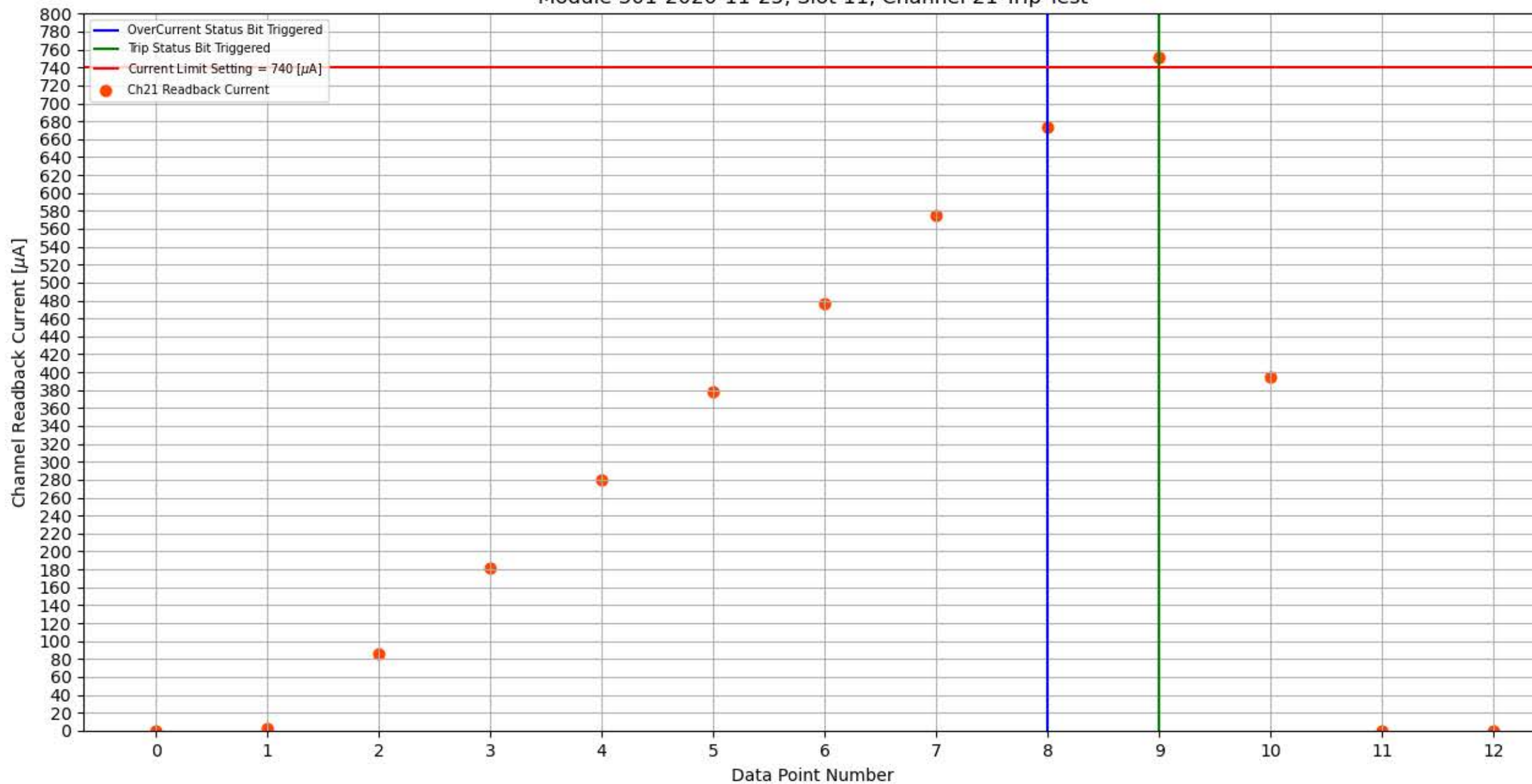
Module 301-2020-11-25, Slot 11, Channel 21 Trip Test
