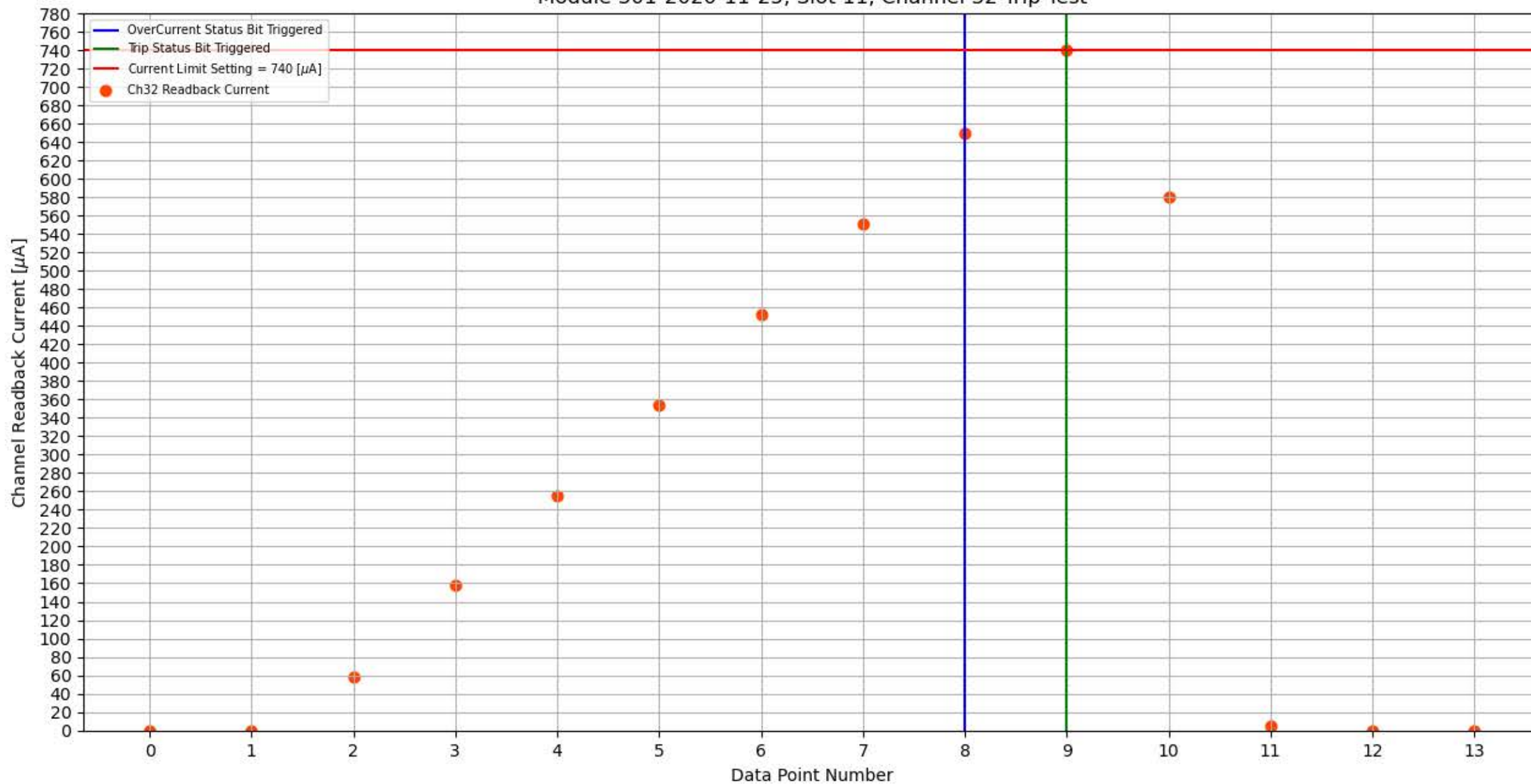
Module 301-2020-11-25, Slot 11, Channel 32 Trip Test
