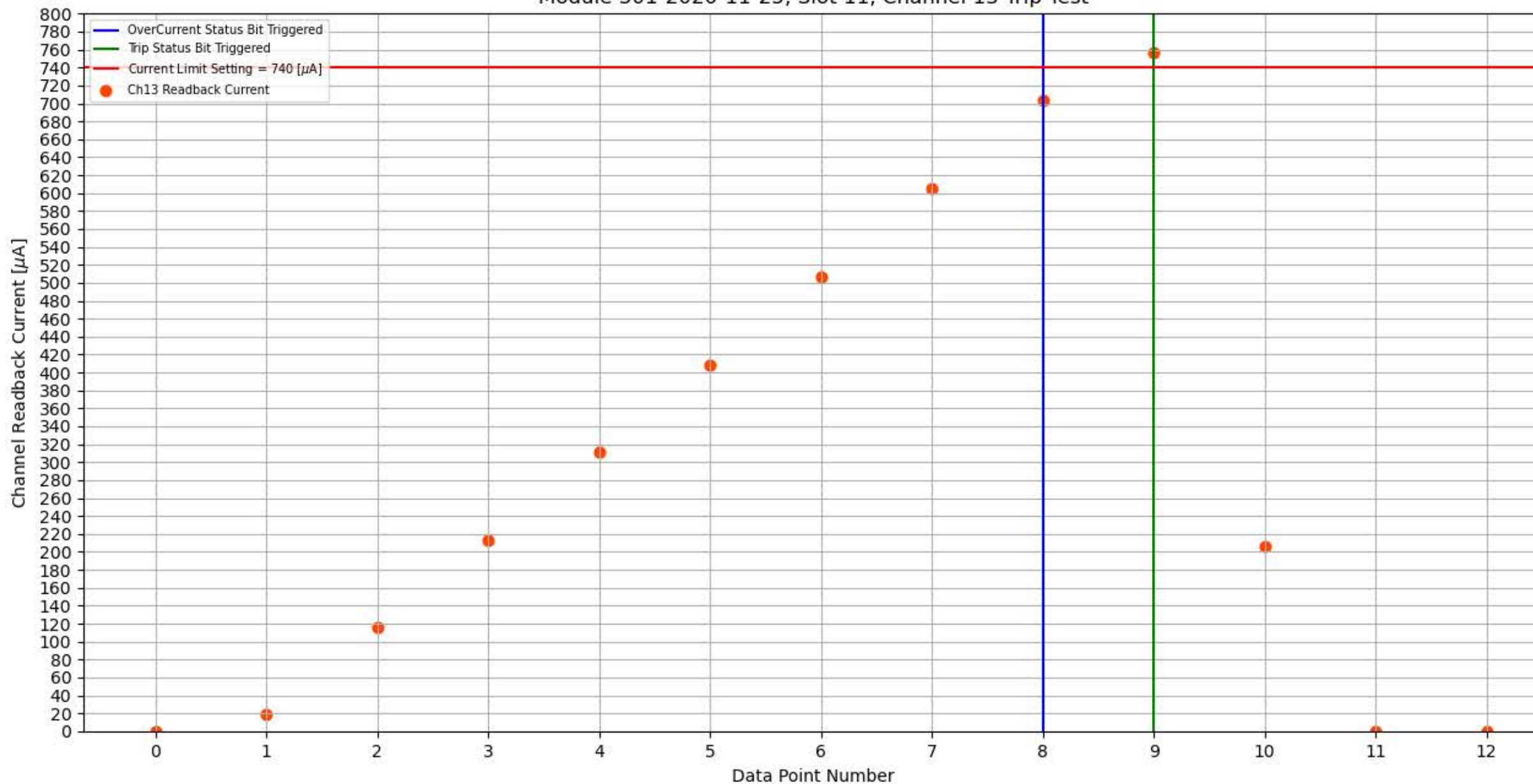
Module 301-2020-11-25, Slot 11, Channel 13 Trip Test
