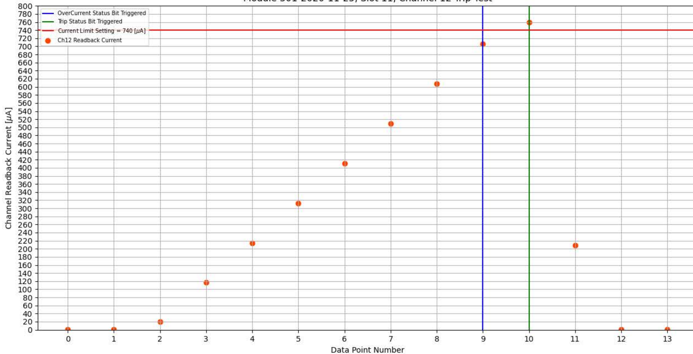
Module 301-2020-11-25, Slot 11, Channel 12 Trip Test
