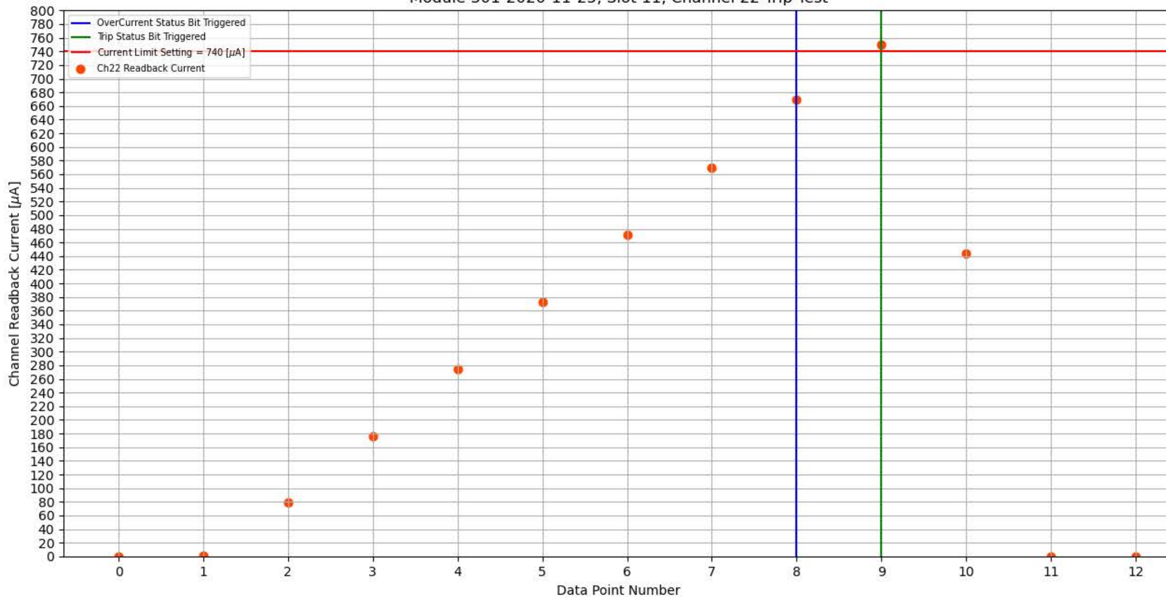
Module 301-2020-11-25, Slot 11, Channel 22 Trip Test
