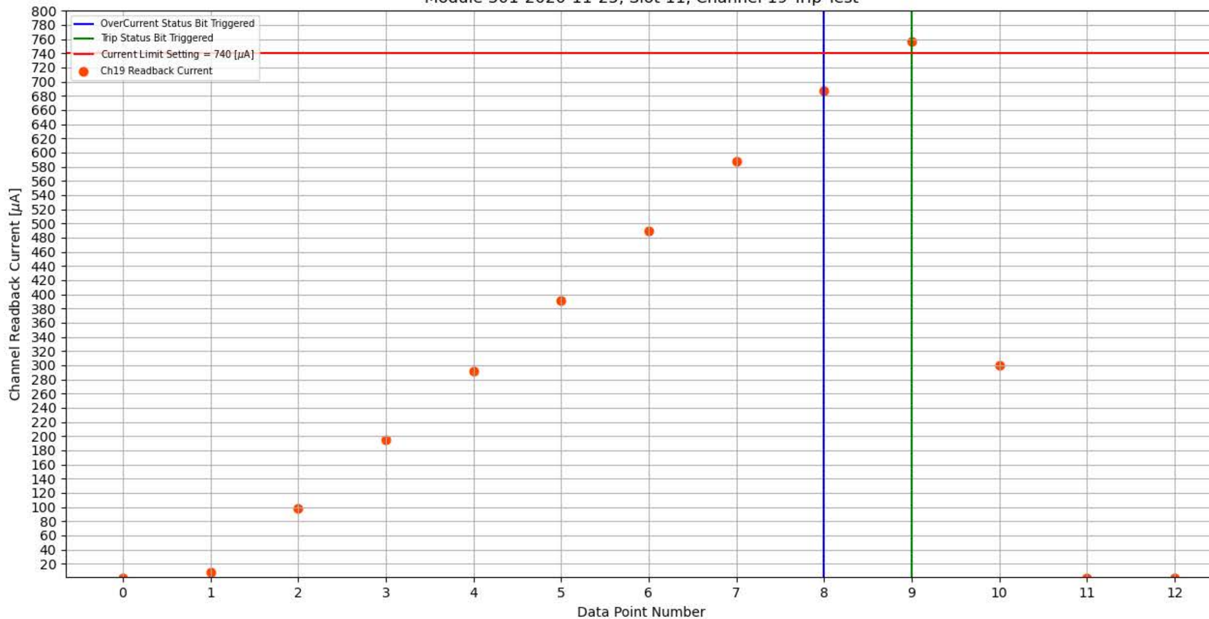
Module 301-2020-11-25, Slot 11, Channel 19 Trip Test
