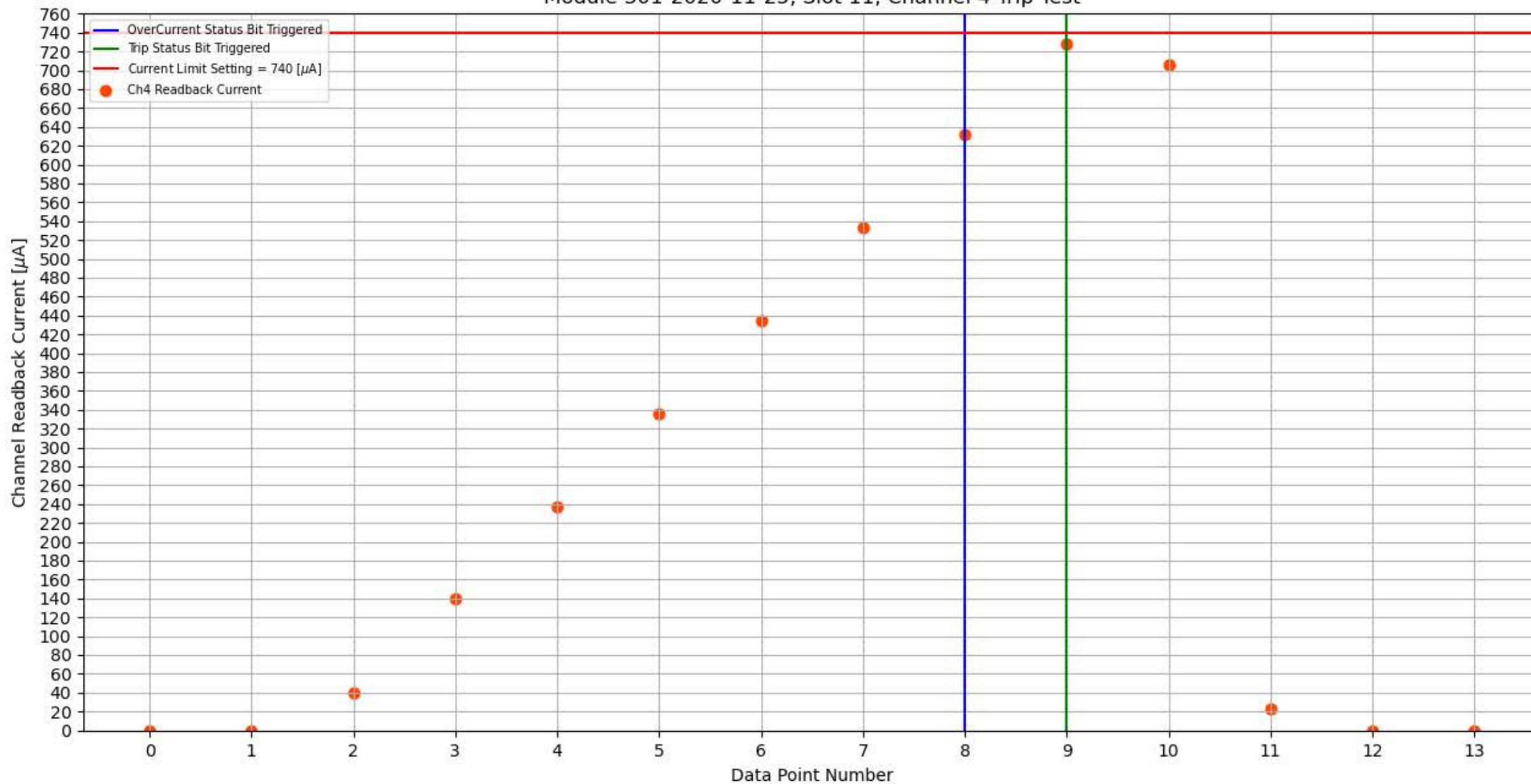
Module 301-2020-11-25, Slot 11, Channel 4 Trip Test
